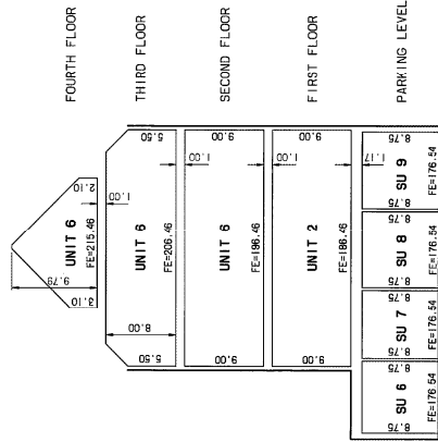
SECTION A-A BUILDING A
