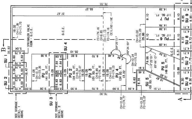
BUILDING A PARKING LEVEL INTERIOR WALLS 0.25 WIDE EXTERIOR WALLS 0.67 WIDE
