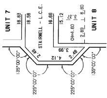
STAIRWELL DETAIL 1 NOT TO SCALE
