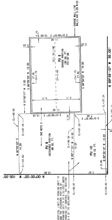
PARKING UNIT DETAIL SCALE: 1" = 5'
