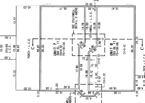
BUILDING B SECOND FLOOR WALLS 0.46 WIDE, OR AS NOTED
