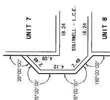
STAIRWELL DETAIL 2 NOT TO SCALE
