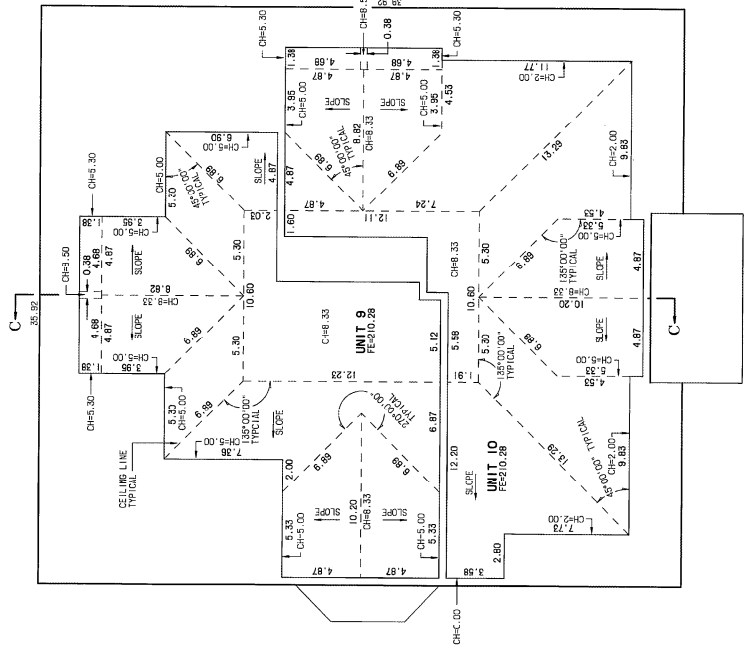
BUILDING B FOURTH FLOOR CEILING DETAIL SCALE: 1/8" = 1'
